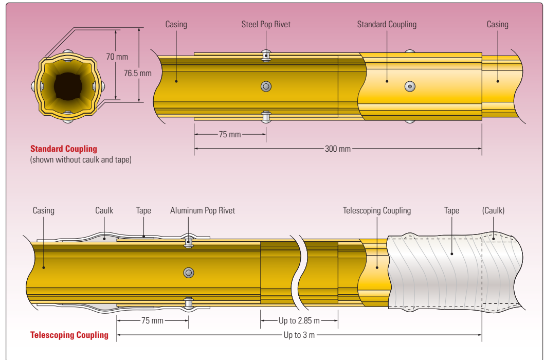
• Illustration depicts the Model 6500 Inclinometer Casing dimensions, and configurations of the standard and telescoping couplings.
