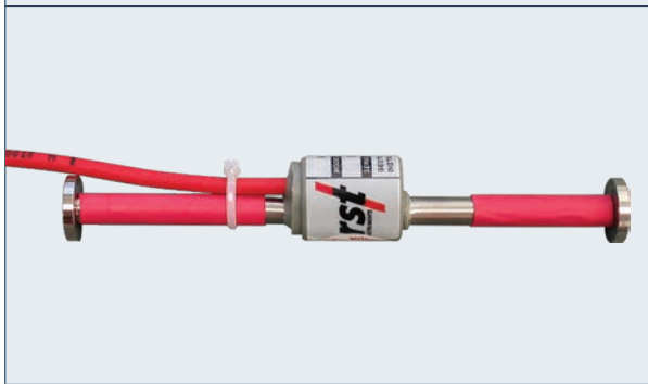
Vibrating Wire Embedment Strain Gauge
